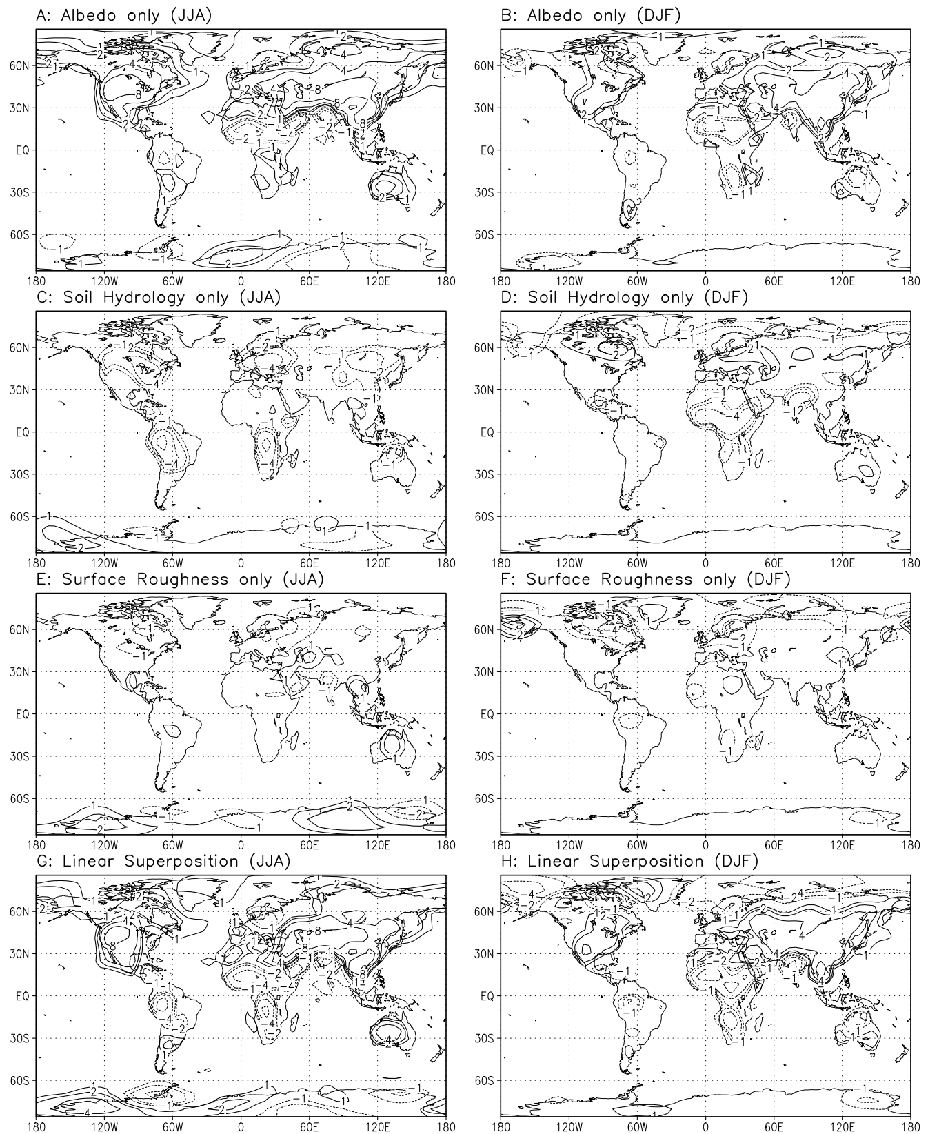
Figure 4: Differences in near surface temperature (in \text{K}^{-1} ) for set-2 (changes of individual surface parameters): Seasonal differences between the green planet and desert world climates for June-August (JJA, left) and December-February (DJF, right). A, B: Changes in albedo only, C, D: Changes in hydrological cycle only, E, F: Changes in surface roughness only, and G, H: Linear superposition. Contours are \pm 1, 2, 4, 8, 16 \text{ K} . Negative contours are dashed.
