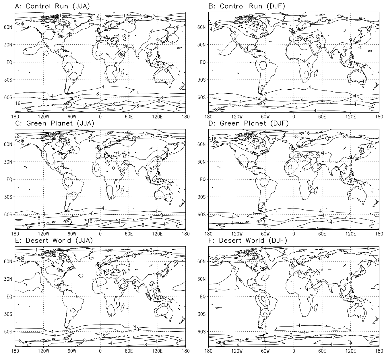
Figure 8: Differences in near surface temperature (in K) for set-4 ( \text{CO}_2 sensitivity): Seasonal differences between two times \text{CO}_2 and present day \text{CO}_2 climates for June-August (JJA, left) and December-February (DJF, right). A, B: Present day vegetation, C, D: Green planet, and E, F: Desert World. Contours are \pm 1, 2, 4, 8, 16 K. Negative contours are dashed.
