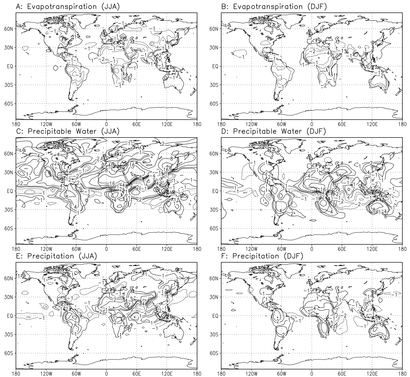
Figure 1: Differences in the water cycle for set-1: Seasonal differences between the green planet and desert world climates for June-August (JJA, left) and December-February (DJF, right). A, B: Evapotranspiration (in \text{mm day}^{-1} ), C, D: Precipitable water (in \text{kg m}^{-2} ), and E, F: Precipitation (in \text{mm day}^{-1} ). Contours are \pm 1, 2, 4, 8, 16 \text{ mm day}^{-1} or \text{kg m}^{-2} . Negative contours are dashed.
