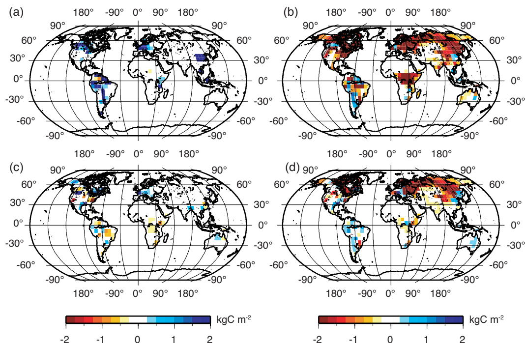
Fig. 4. Differences in vegetation biomass for (a) “full vegetation” – “bare ground” initializations for n=2 (b) same as (a), but for “full vegetation” initialization – “Control”, (c) and (d) are the same as (a) and (b), but for n=8 .
