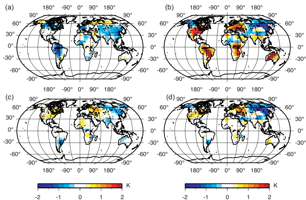
Fig. 5. Same as Fig. 4, but for Northern Hemisphere springtime (March–May) near surface air temperature.
